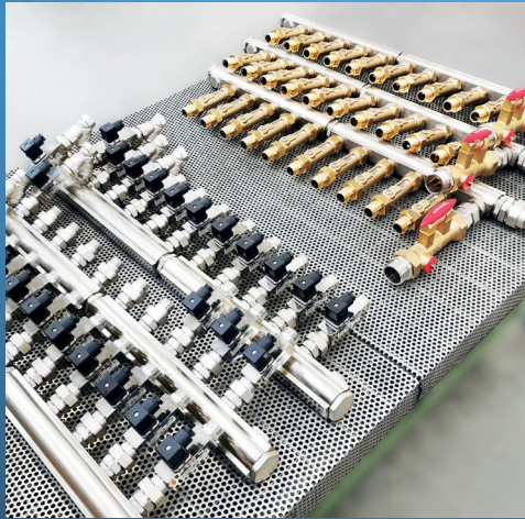
Hydraulic distribution manifolds designed upon customers' requests.
